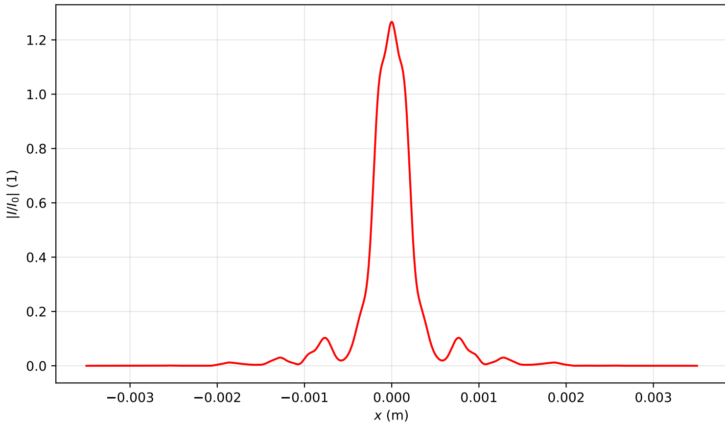
Intensity profile I(x, y = 0, z = 1.672)/I_0 , P_{in}=5.5P_{cr} , artificial time
